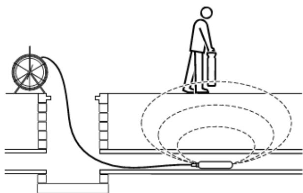
Figure 9.7 Sonde deployment
