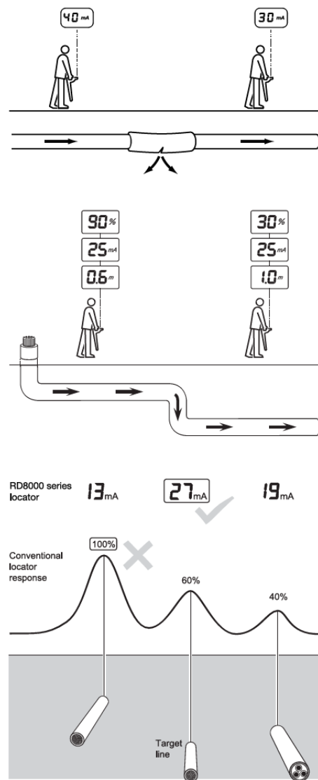
Figures 6.4 – 6.6 Taking current readings
