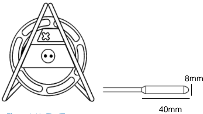
Figure 9.10: FlexiTrace
