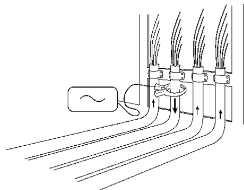
Figures 9.5 – 9.6: Connecting transmitter clamps
